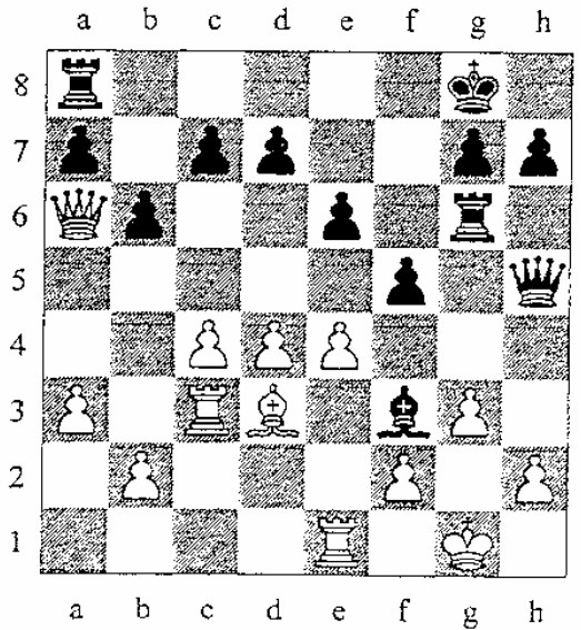
Diagram 3 Ambramovich-Botvinnik Leningrad 1924
