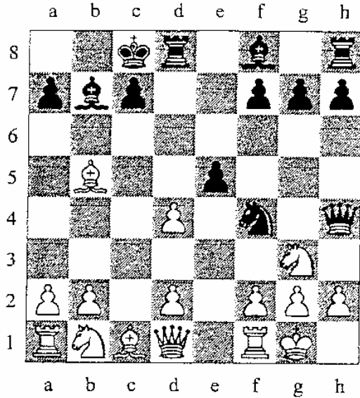
Diagram 3 Ambramovich-Botvinnik Leningrad 1924
